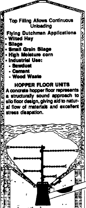
FLYING DUTCHMAN UNLOADER WITH HOPPER FLOOR
