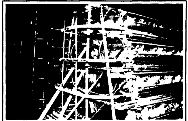
LUBING Nipple Waterers With Auto High Pressure Flushing System To Outside Of Building. LUBING Nipples Have An Unconditional 10 Year Warranty.
