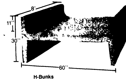
H-Bunks
