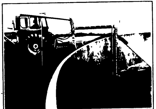
MAXI-PUMP installed with vacuum hose, hydraulic directional trap, agitator kit and filling pipe to agitate and pump liquid hog manure
