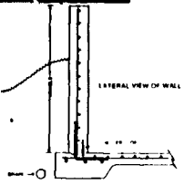
POURED IN PLACE CONCRETE TANKS
