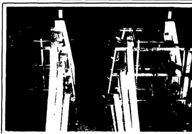
CHORE-TIME® Dual Auger Fill System CHORE-TIME® Rubber Finger Soft Touch Variable Speed Collectors With CHORE-TIME® 4 High Dura Cage System And Nipple Waterers
