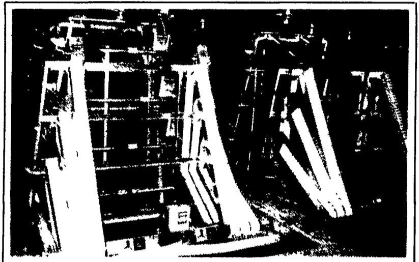
CHORE-TIME® Dual Auger Fill System CHORE-TIME® Rubber Finger Soft Touch Variable Speed Collectors With CHORE-TIME® 4 High Dura Cage System And Nipple Waterers
