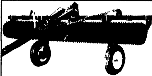
BRILLION 12 FT. PACKER WITH TRANSPORT Machine Weight Is Hydraulically Rotated Over Wheels For Easy Transport
