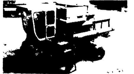
Case IH 1660 Combine, 1988 Yr., 901 Hrs., 2 Spd. Hydro Trans., Auto Header Height Control, Grain Loss Monitor, Feeder Reverser, Rock Trap (U6205)
