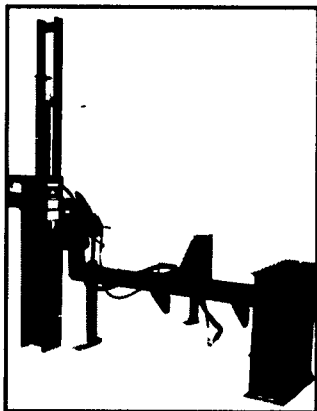
Post driver with optional offset drives posts in corners or in close quarters where center mounted driver can't reach.
