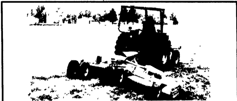
Features 5-Foot Center Section And 5-Foot Right Wing. Cuts A 10-Foot Swath. Ideal For Roadside Mowing.
