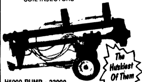
H5000 PUMP - 23000 LPM (6000 GPM) 20 TONS PER MIN., CAN BE CHANGED FROM "PUMPING" TO "AGITATING" AT FULL SPEED
