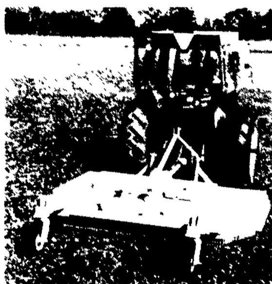
Model M121 mounts on standard category 2, 3-point hitch Model illustrated with optional equipment.
