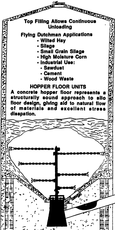
FLYING DUTCHMAN UNLOADER WITH HOPPER FLOOR
