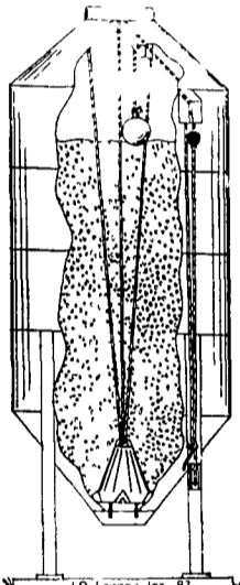
"DIRECT READING" - BIN LEVEL INDICATOR
