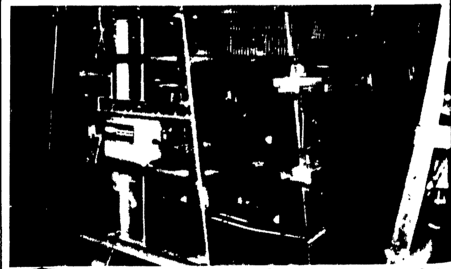
CHORE-TIME ® ULTRAFLO ® Feeding System With Feeder Outside Of Cage Where It Belongs, And New Adjustable Cage Front
