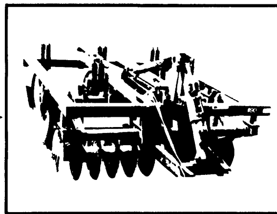
MODEL 890 COULTER CHISEL WIDTH—6' 9" to 16' 9" WEIGHT—3140# to 7790#
