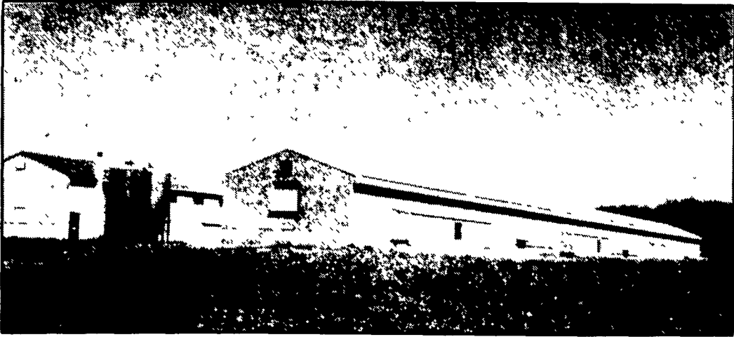
36'x340' High-Rise Building With Fan Sheds And Brown-Out Air Inlet Overhangs
