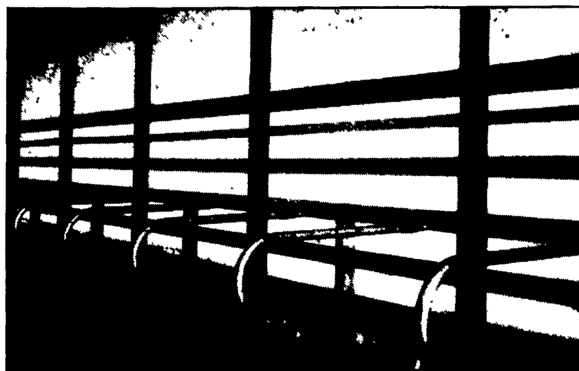
Treated 6x6 Post Every 8' O.C. With Short 4x6 Post Between To Secure Stalls
