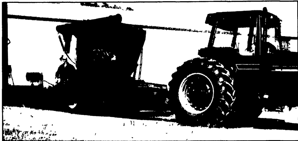
385 Utility 2WD 35 PTO hp (26.1 kW)
