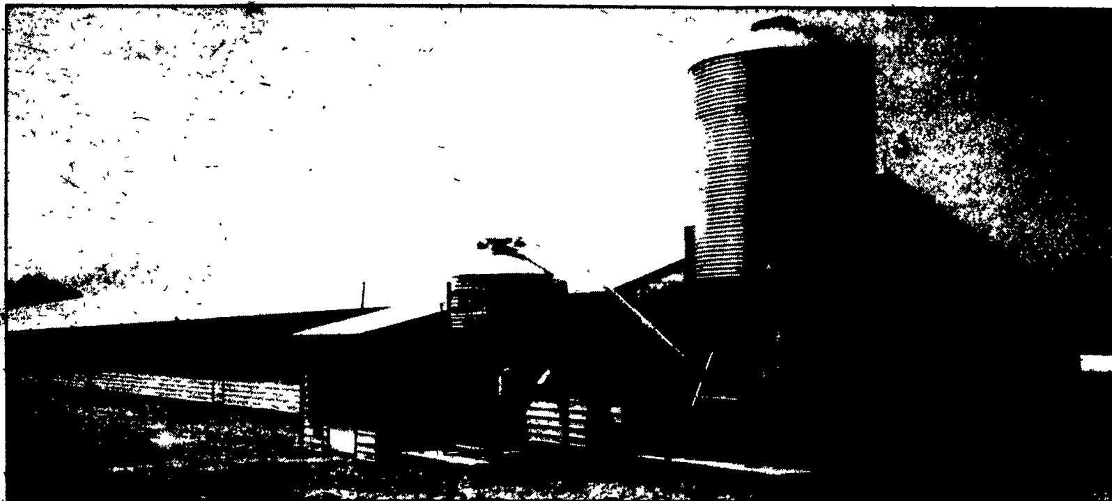
42' x 300' Single Story Building With G&M Blackout Light Restrictors And CHORE-TIME ® Storage Bin With Automatic Weighing System.
