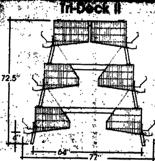
High density in the proven low profile cage design. Available in 8-foot or 10-foot cage sections. Cage size options: 12"x20", 15"x20", 16"x20" and 24"x20".
