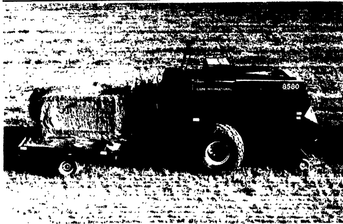
The Model 8580 baler from Case IH is a highly automated, electronically controlled machine that offers peak productivity to the large-volume hay grower. Attached to the baler is the Model 8581 bale accumulator trailer that also is electronically controlled. The baler producer 46.5x50x108-inch bales weighing up to 2,000 pounds.
