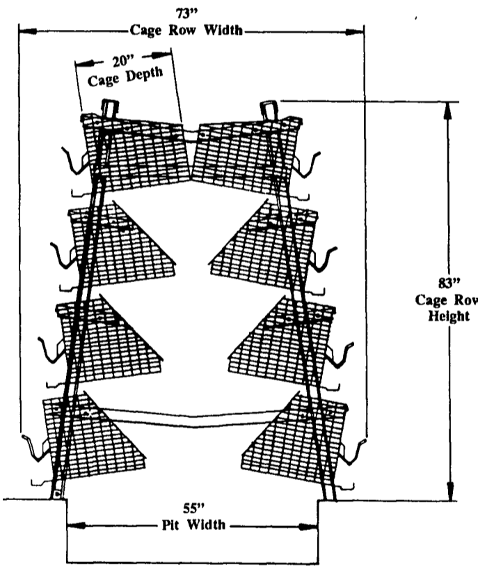
CHORE-TIME New 4 Tier High Cage System With CHORE-TIME Ultraflo Feeding System
