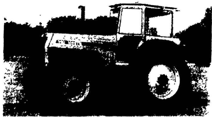
The White 140 row-crop tractor is rated at 137 pto horsepower at 2200 rpm. It has a six-cylinder, 359 C.I.D. Cummins "B" diesel engine.
