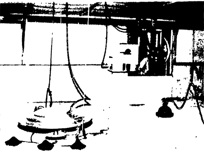
50'x520' Starter & Grower Turkey Building, Starter Building With Wood Trusses, Tri Ply Ceiling, Insulated Sidewalls.
