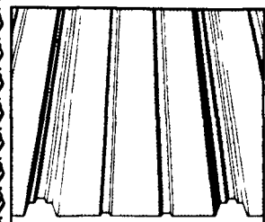
GRANDRIB 3 GALVANIZED STEEL Grandrib 3 has a full 36" coverage with 1/4" deep ribs every 9". The rib's depth and placement give it exceptional rain carrying capacity. Anti-siphon side lap makes it virtually leak proof.
