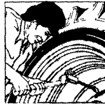
To secure the Circoloc dual, use the handle furnished to snap over the levers on the clamps. To assist in removing duals, position one of the clamp levers top center and use the handle to loosen the clamps by applying leverage toward the tractor. Loosen the top clamp last.
