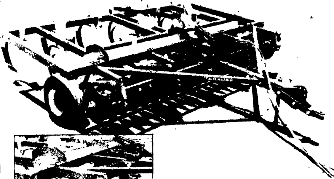
Hydraulic coultter assembly features spring-mounted bearing arms to flex over buried rocks.
