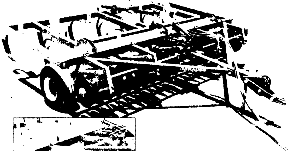
Hydraulic coultter assembly features spring-mounted bearing arms to flex over buried rocks.
