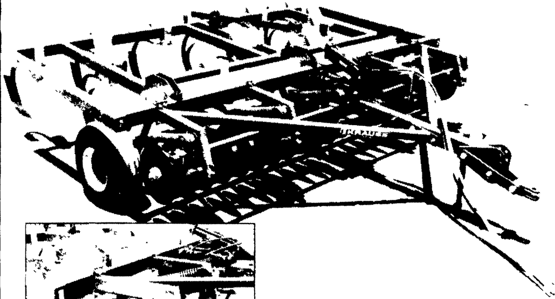
Hydraulic coulters assembly features spring-mounted bearing arms to flex over buried rocks.
