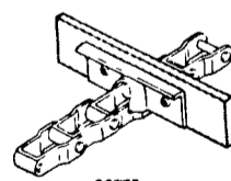
667H SINGLE CONVEYOR CHAIN WITH RUBBER PADDLE
