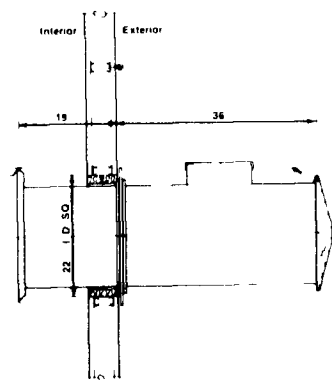
The XL1800 mounts through either endwalls or sidewalls. It's suspended by twin guy wires for easy installation without mounting brackets to get in the way.
