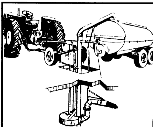
Agitator/Filler Pump
