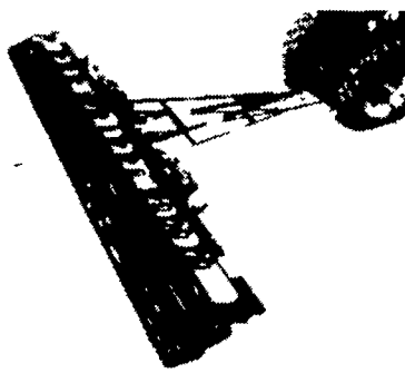
A single cylinder operates both the cultivator and the grain drill. Depth of cultivator and drill can be set independently.
