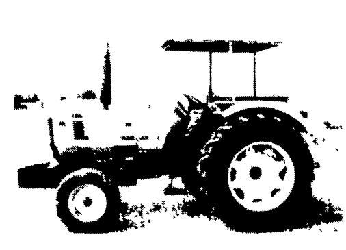
DX 3.30 51 HP, 8F/4R Syncromesh Transmission, Differential Lock, Independent 540 PTO, Cat. I 3 Pt. Hitch, 5,291 Lb. Lift Capacity, 13.5 GPM Hydraulics
