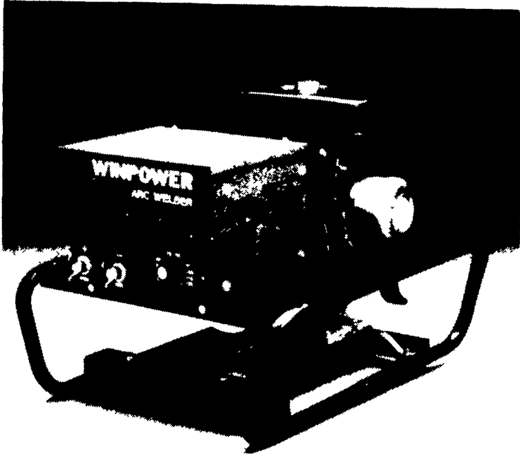
Winpower Corp's new 135-amp portable DC arc welder.
