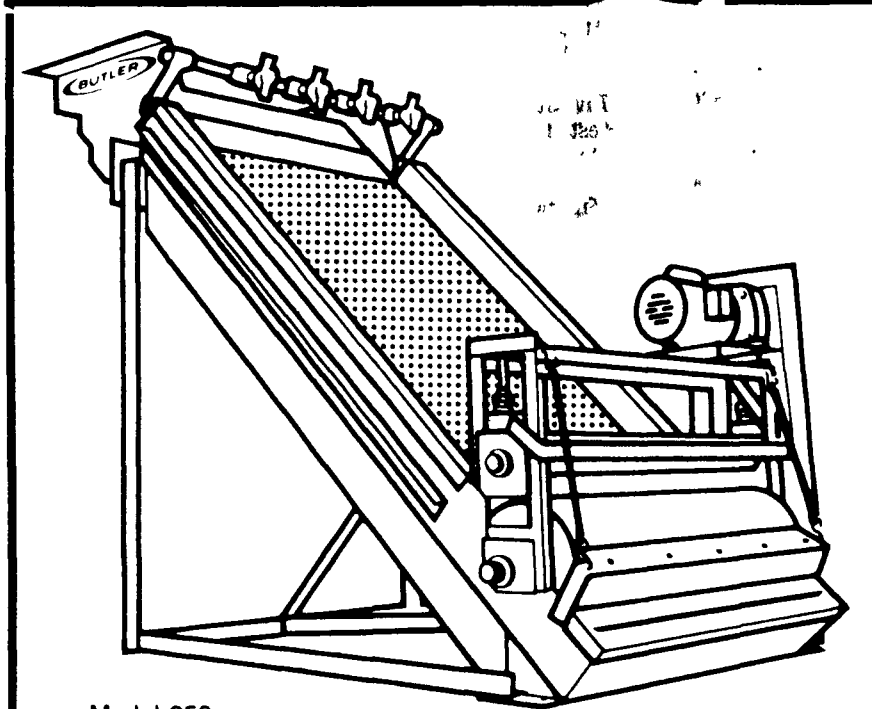
Model 250. Capacity: 250 GPM (gallons per minute.)
