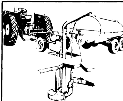
Agitator/Filler Pump
