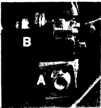
Two adjustment bolts (A B) for single station cutterbar adjustment
