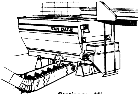
Stationary Mixer
