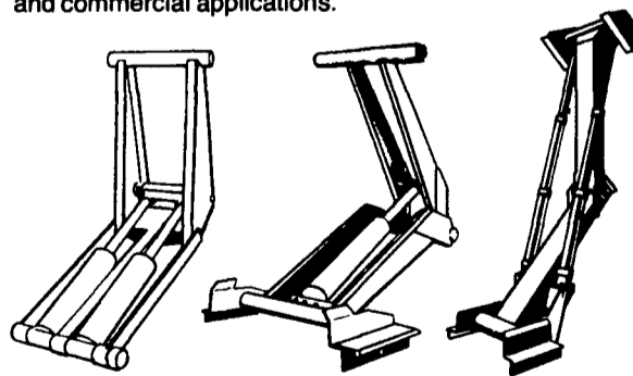
TRI-LOADER European-style contractor body with hinged sides and double-acting tailgate
