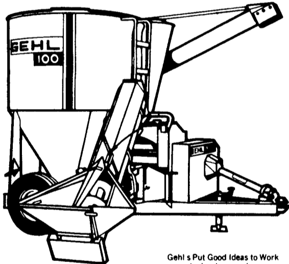
Gehl's Put Good Ideas to Work in a hydraulic grinder mixer for less maintenance, easier operation. The 100 bushel Mix All unloads as quickly as 3 1/2 minutes. Features include the big 21" mill with 66 reversible hammers, hydraulically driven in feed attachments with infinite speed control and quick change screens for faster performance and operating convenience. Stop by and see the hydraulic 100 Mix All today!
