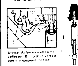
Orifice (A) forces water onto deflector (B). Lip (C) diverts it down to suspend feed (D).
