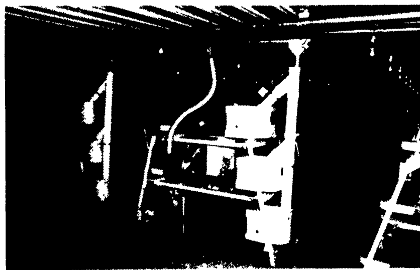
P.V.C. Drop Tubes To Feeders, Flat Chain Feeding System, 2x6 Open Slatted Walkways, Fiberglass Dropping Boards
