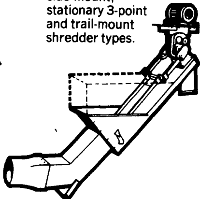
Volume-Belt® center charge feeder.
