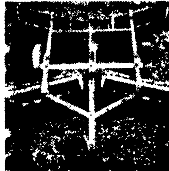
TRANSPORT DISK 10' Cut , 7 1/2" Blade Spacing, 32 Blades 16"-18", Good Paint, Adj. Gang Setting $650
