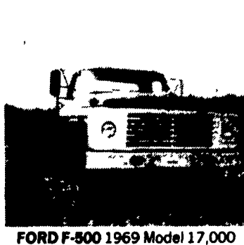
FORD F-500 1969 Model 17,000 GVW Engine, 330 V-8, 4 Speed Trans., Motor Overhauled, Tires - 7:50x20 Mud & Snow on Rear, All Tires 50%, 8'x13' Steel Bed w/Tool Box & Stake Pocket $2,195
