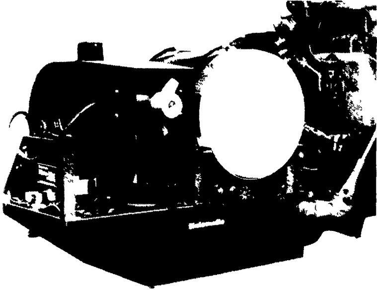
Micronizer spray head and mist sprayer from Automatic offers controlled droplet application without use of booms or motors.
