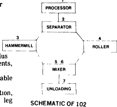
SCHEMATIC OF 102
