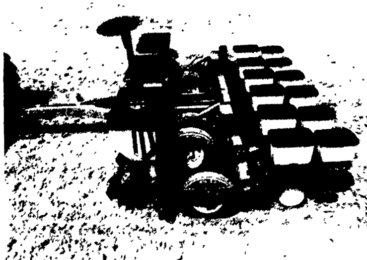
Double frame planter from New Idea features durable construction with two 7-inch steel box beam tool bars.
